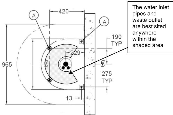
PLAN VIEW OF PEDESTAL UNIT
