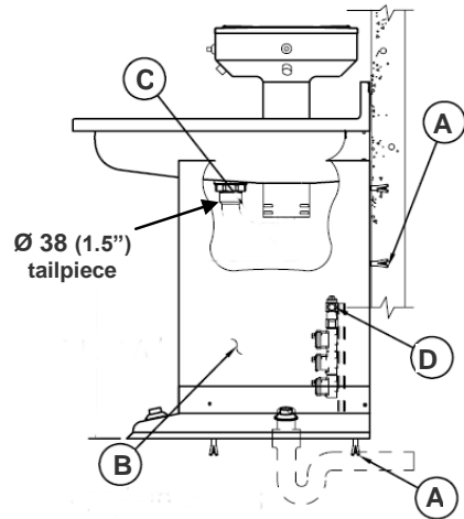
ELEVATION VIEW OF 364 FOUNTAIN WITH FOOT PEDAL
